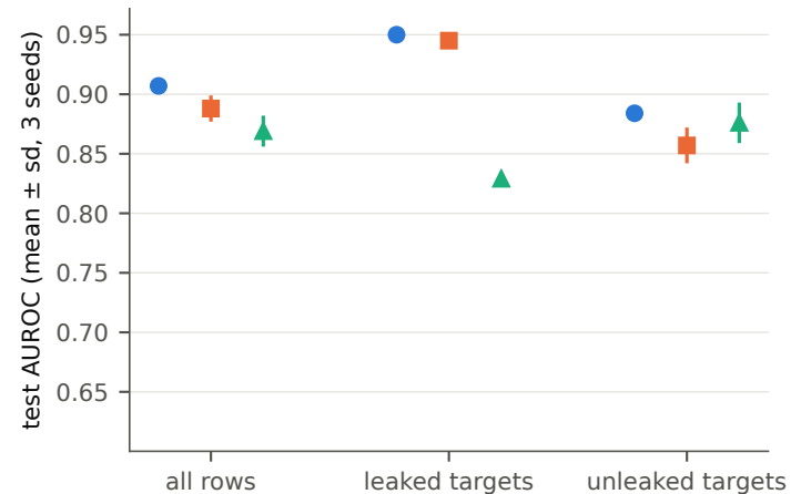
DeepDTA, DAVIS cold-target
