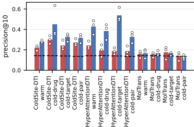
KLIFS ATP pocket
