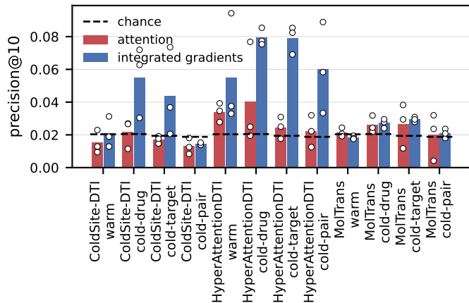
UniProt annotated residues
