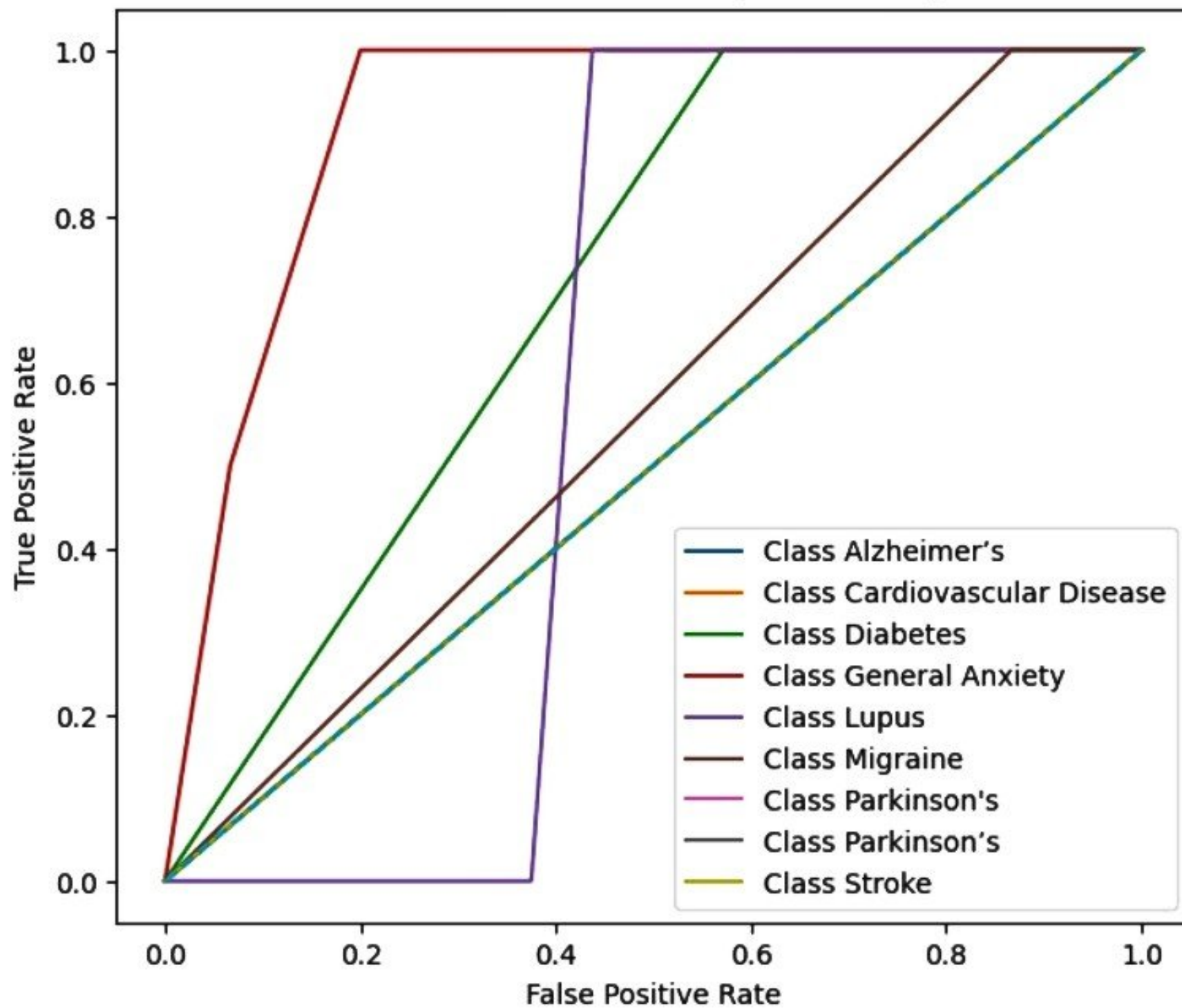
Multiclass ROC Curve (AUC = 0.59)
