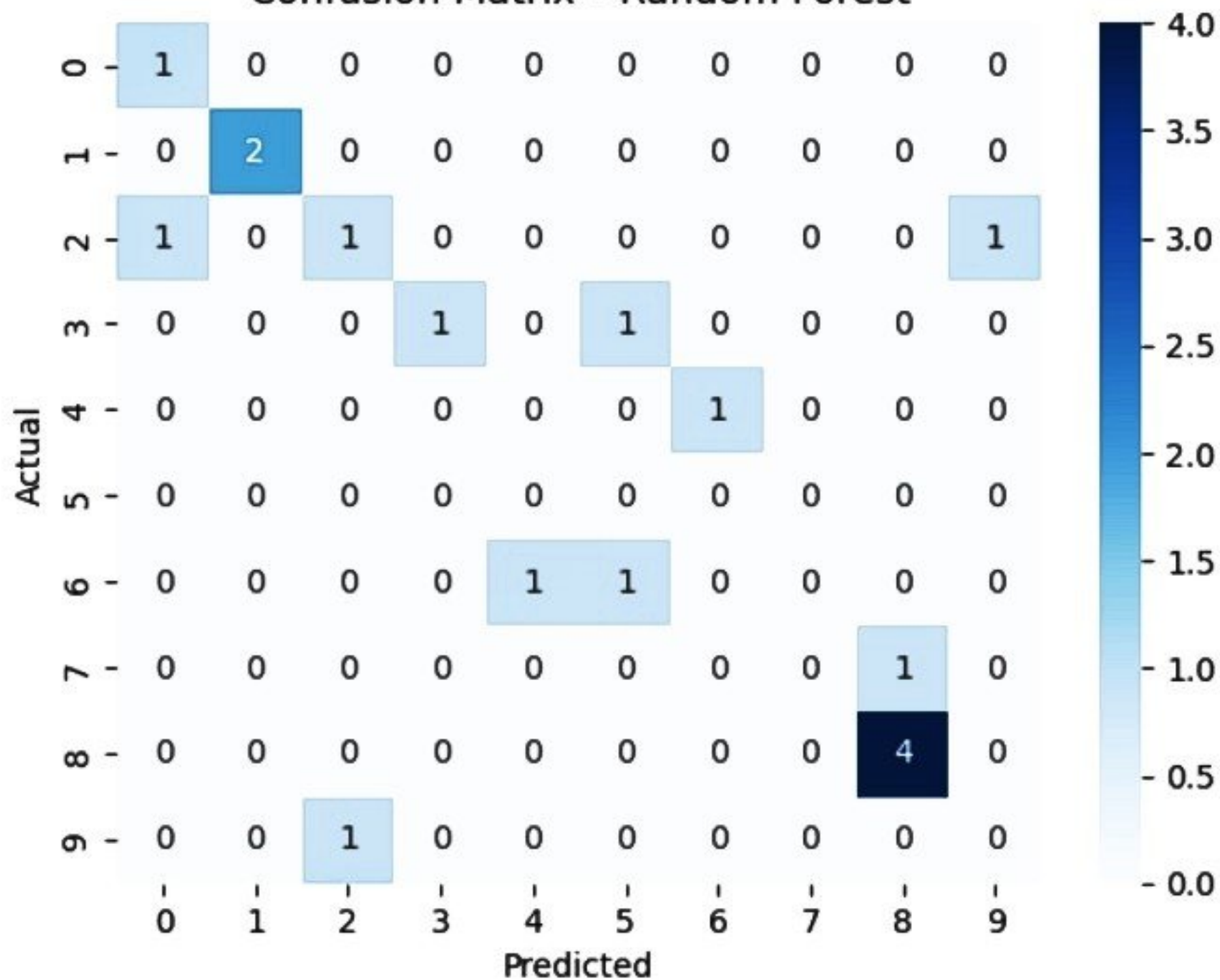
Confusion Matrix - Random Forest
