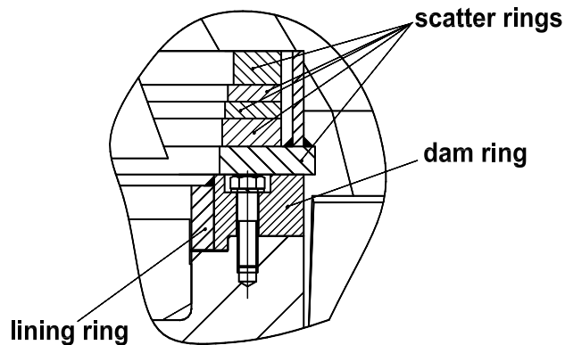
Fig. 1 principle sketch
