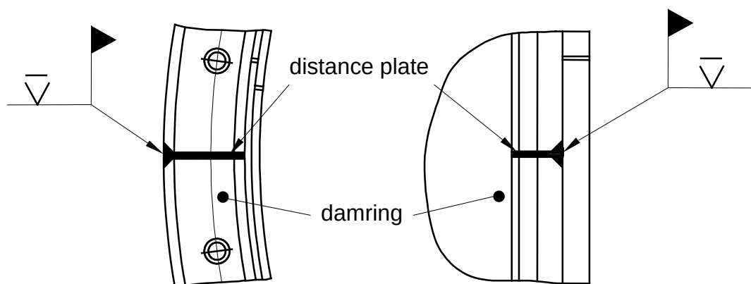
Fig. 2 principle sketch
