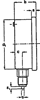
TYPE A Lower Connection - Stem Mounting.
