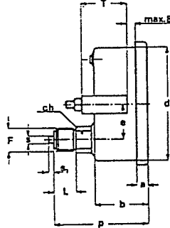
TYPE B Back Connection - Flush Mounting, U-Clamp.
