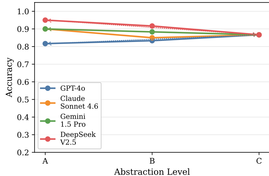
Accuracy: Abstract \rightarrow Situated Gradient
