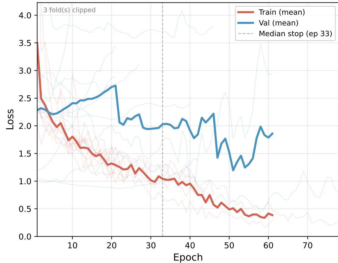
GNN (Pretrained) — Receiver (Stage 1)
