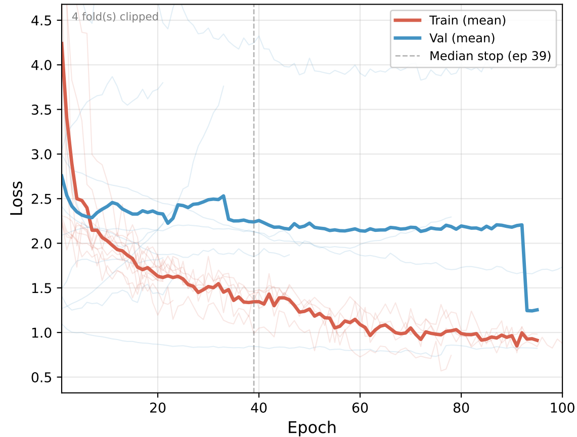
GNN (Pretrained) — Receiver (Stage 1)
