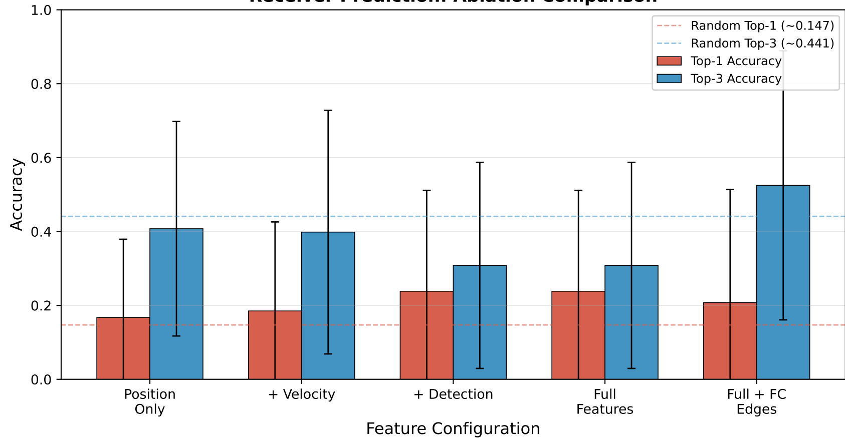
Receiver Prediction: Ablation Comparison
