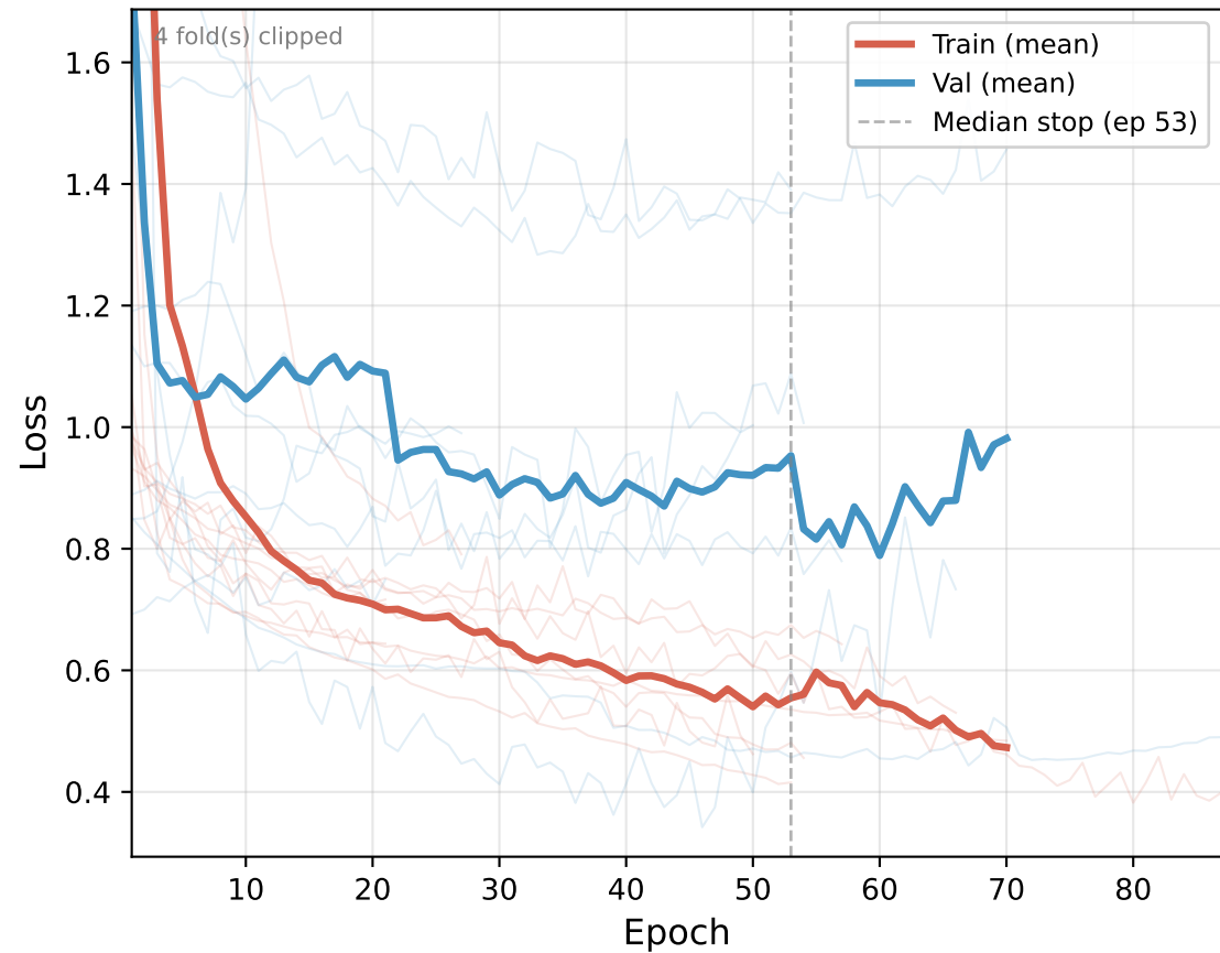
GNN (Pretrained) — Shot (Stage 2)
