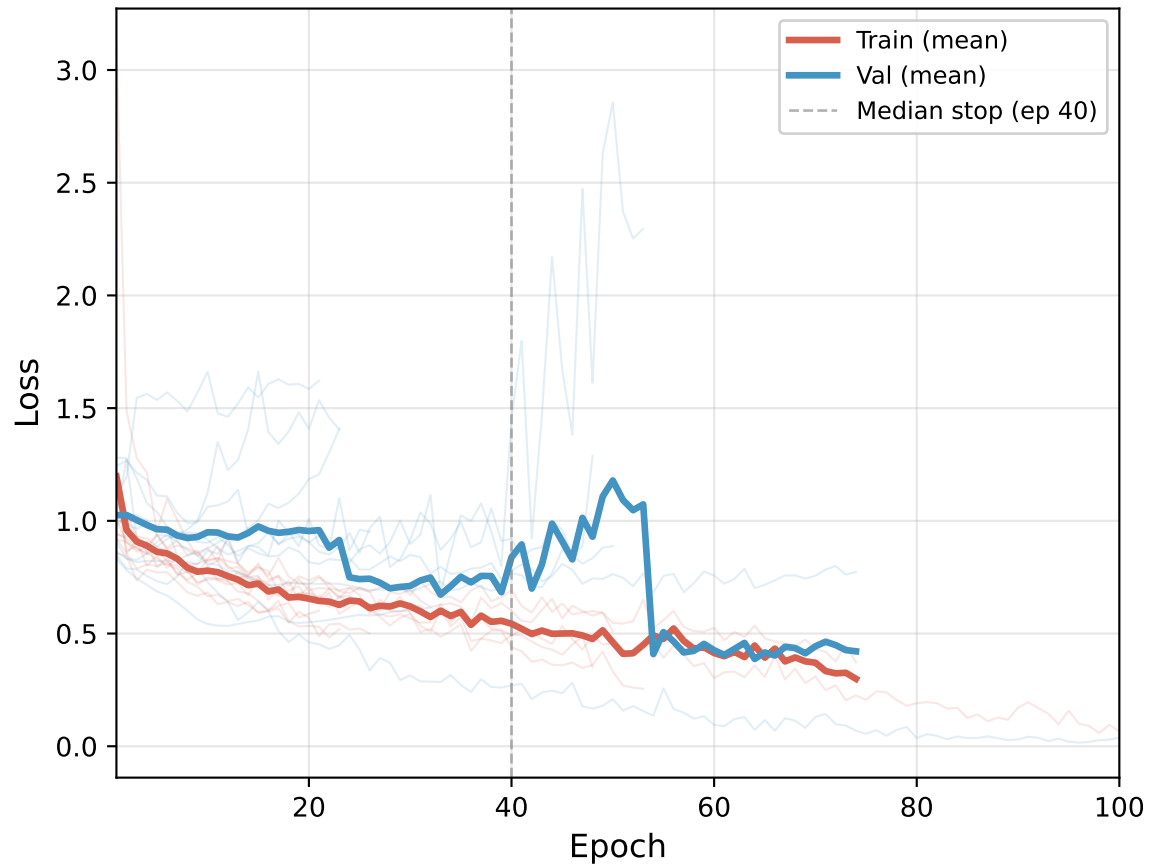
GNN (Pretrained) — Shot (Stage 2)
