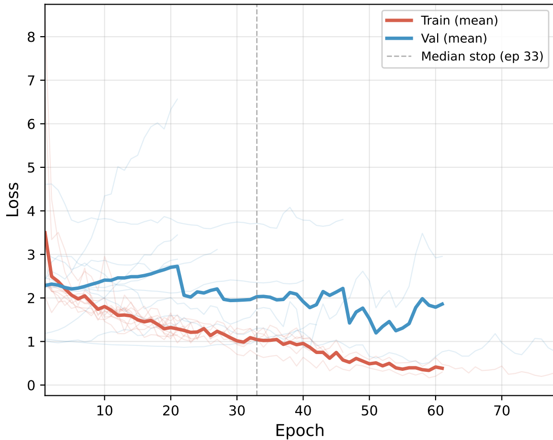
GNN (Pretrained) — Receiver (Stage 1)
