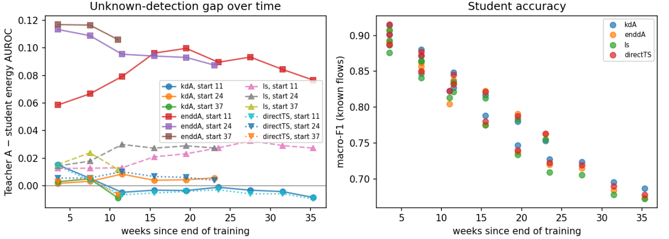
Fig. 2. Left: teacher-minus-student energy AUROC against weeks since the end of training, per student condition and start date. The gap for kdA and directTS shrinks and crosses zero; for ls it grows; for enddA it stays large. Right: student macro-F1 over the same axis, showing the drift all models suffer.
