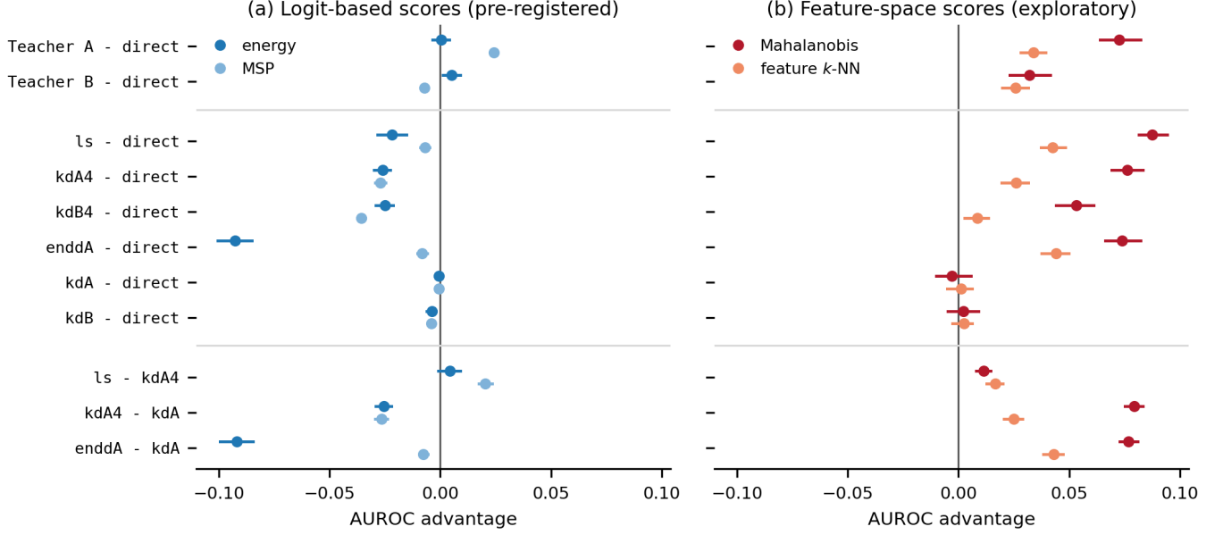
Fig. 5. Unknown-traffic detection advantage over the directly trained student, by scoring rule (exploratory; 18 test windows): (a) the pre-registered logit-based scores; (b) the feature-space scores. Markers are pooled estimates, bars are 95% cluster bootstrap intervals, and both panels share one scale. The top block compares models of different feature dimensionality and is indicative; the lower blocks compare identical architectures.
