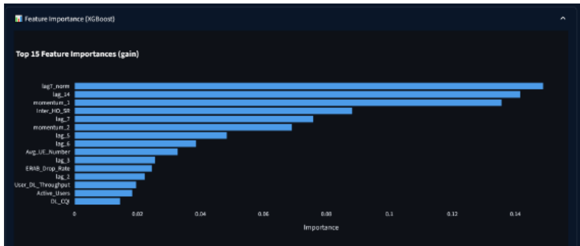
Figure 5.6: Top-15 XGBoost feature importance by gain for DL Traffic Volume forecasting. lag7_norm and lag_14 dominate, confirming strong weekly periodicity. Cross-KPI features ( Inter_HO_SR , Avg_UE_Number ) and momentum terms contribute non-linear explanatory power.
