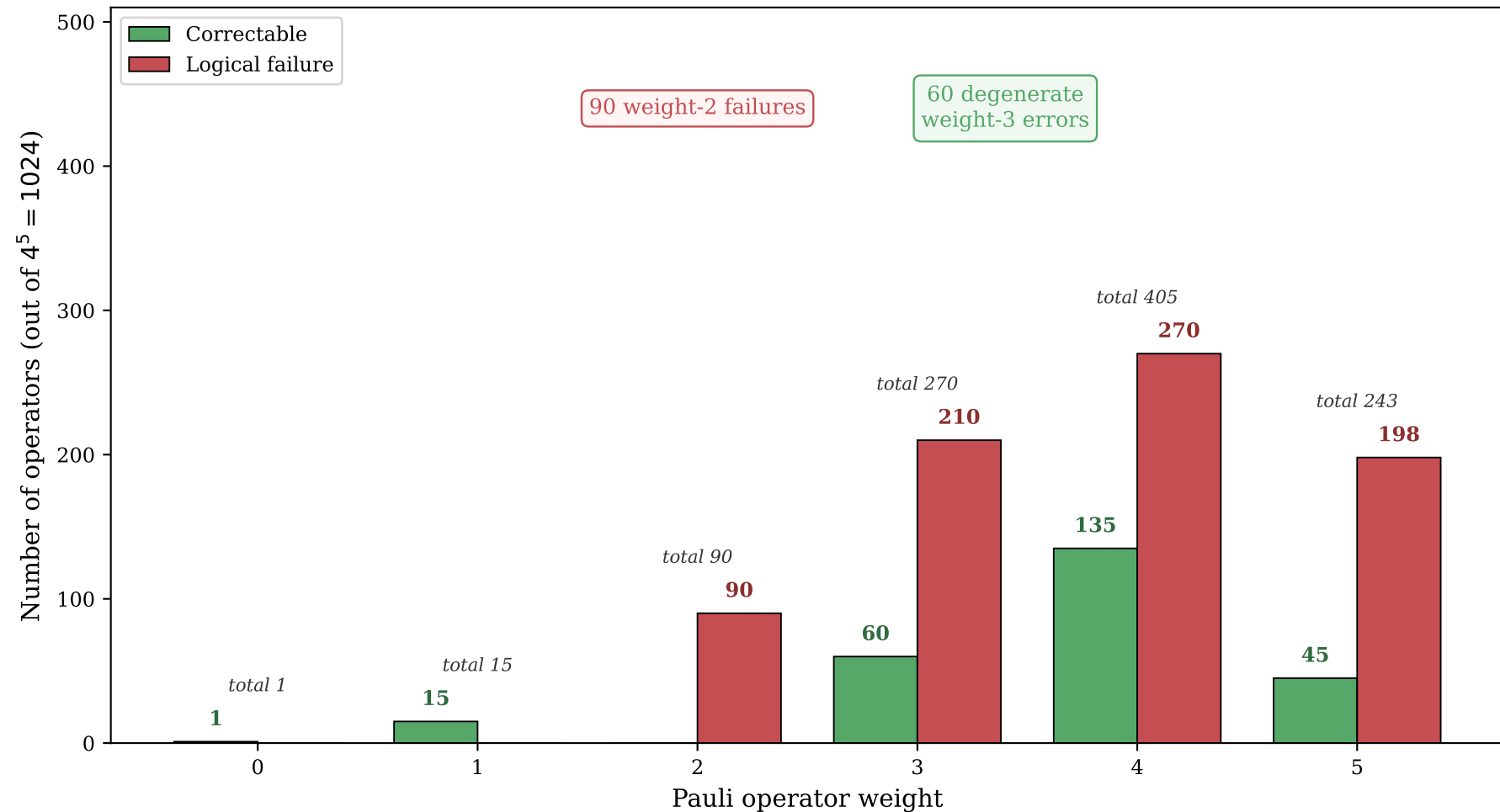
Complete Pauli weight distribution for the [[5, 1, 3]] code
