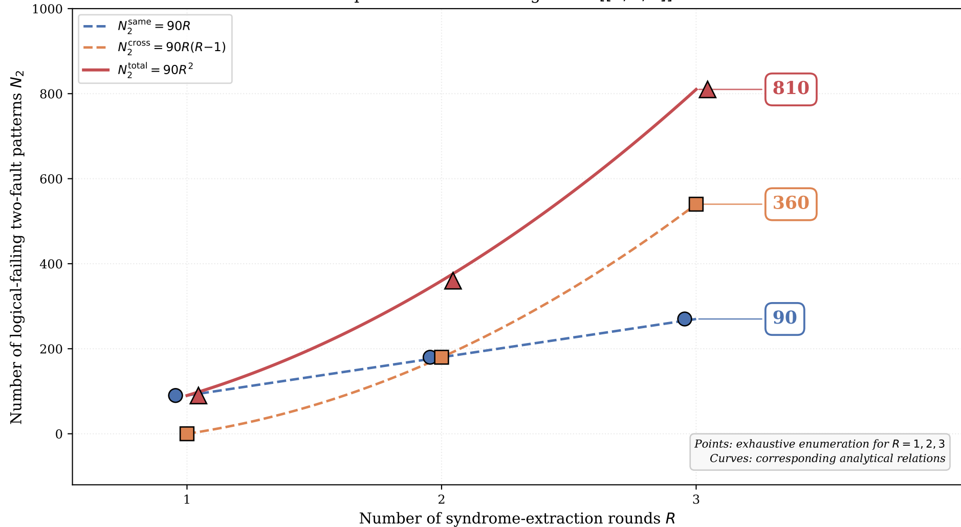
Temporal two-fault scaling of the [[5, 1, 3]] code
