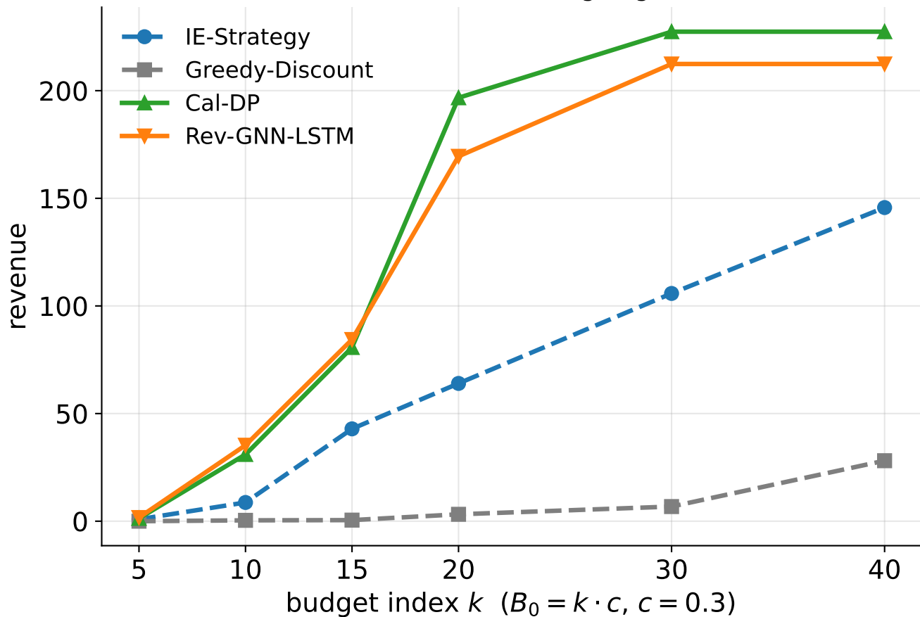
Modular-FF (n=500, avg deg 16.6)
