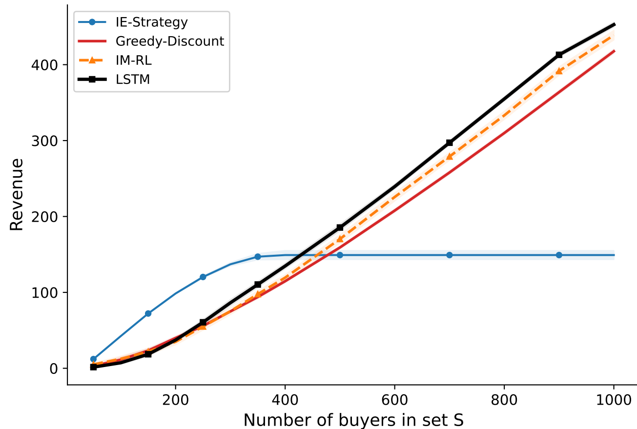
(a) Monotone Concave
