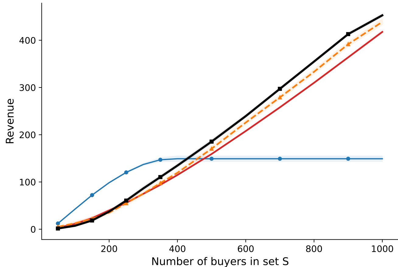
(b) Non-Monotone Concave
