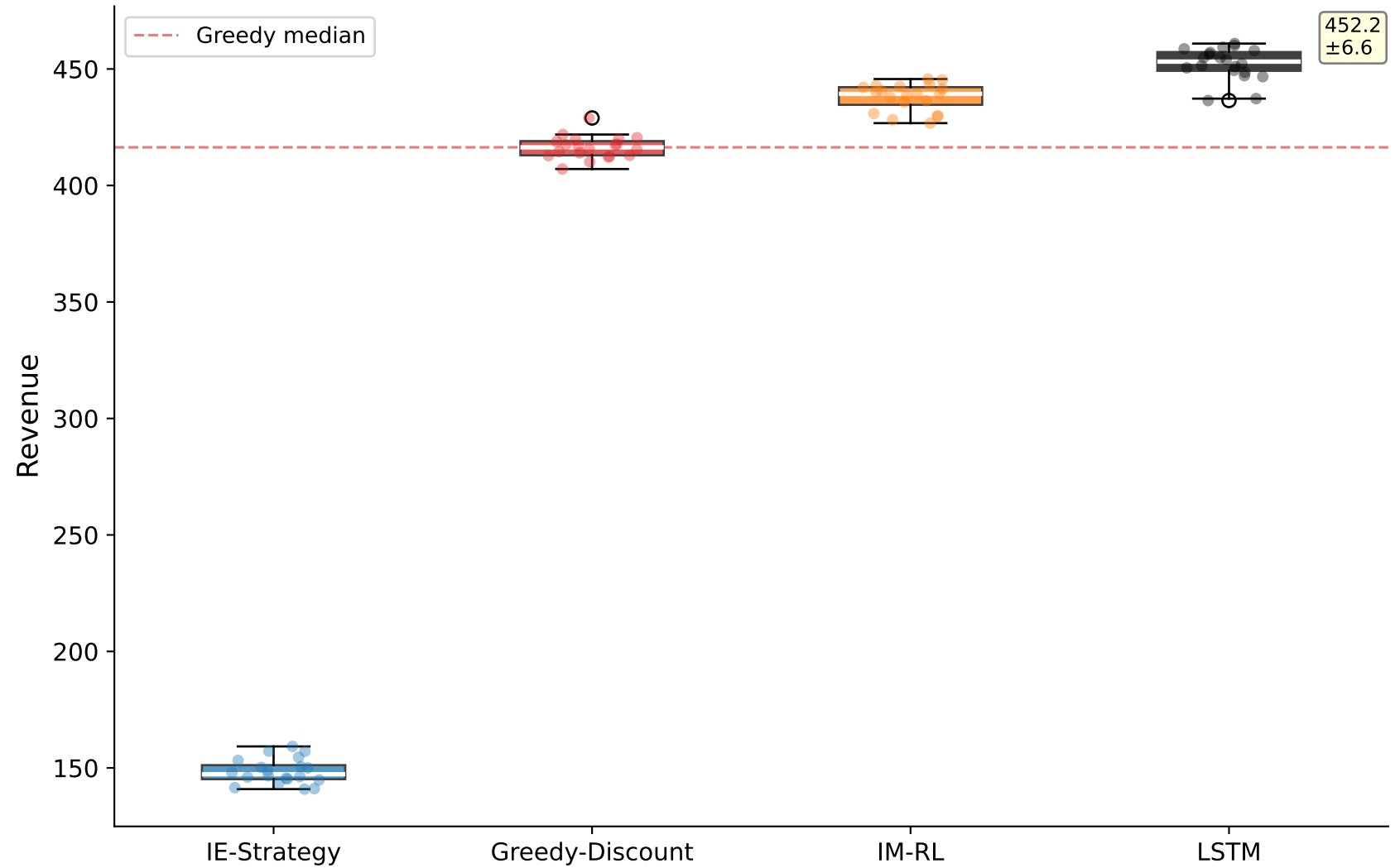
Revenue Comparison (20 seeds, FF n=1000)
