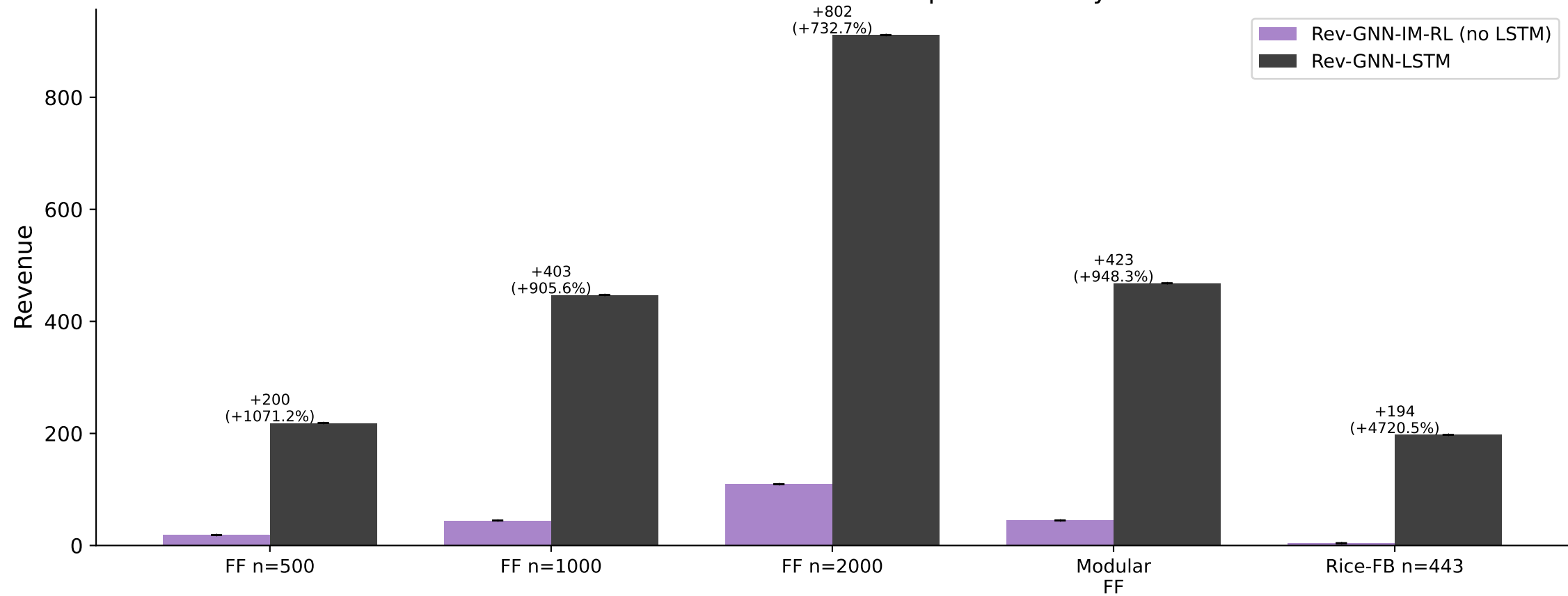
Ablation: Effect of LSTM Temporal Memory
