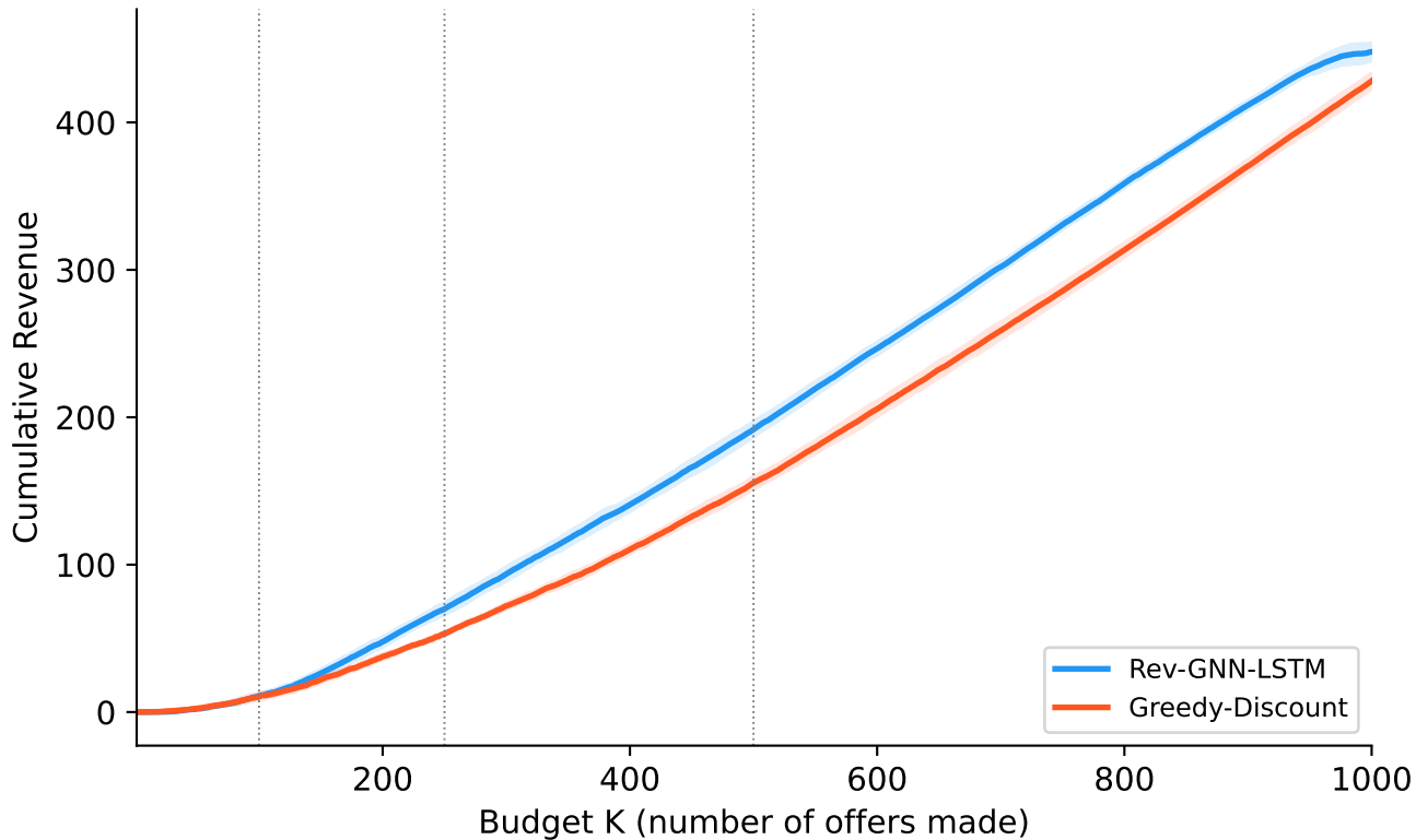
Revenue vs Offer Budget K (FF n=1000, 5 seeds \pm std)
