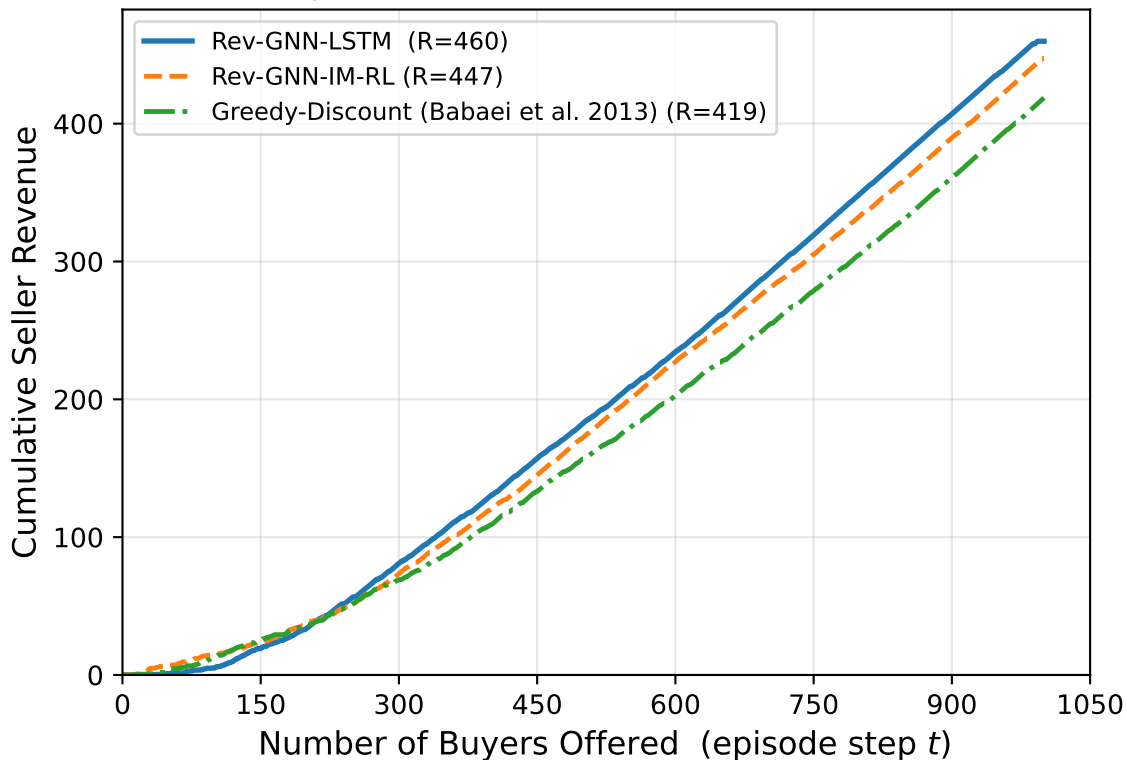
Revenue vs. Buyers Offered (submodular curve, FF-1000 seed=42)
