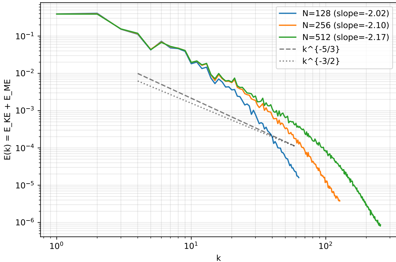
Orszag-Tang 2D MHD turbulence spectrum at t=0.5
