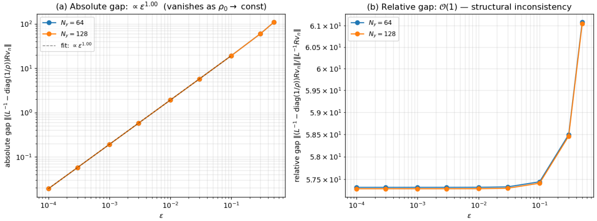
Figure 5.2. Proposition 1 scaling law. Left (a): absolute gap \|(L^{-1} - \text{diag}(1/\rho_0))RV_n\|_2 scales as \varepsilon^{1.00} (log-log slope 1.000, N_y = 128 , \varepsilon \leq 0.1 ), confirming c(\rho_0) \propto \|\rho'_0\|_\infty as \varepsilon \rightarrow 0 . The Boussinesq regime is recovered in the limit. Right (b): relative gap \|(L^{-1} - \text{diag}(1/\rho_0))RV_n\|_2 / \|L^{-1}RV_n\|_2 is scale-invariant at \approx 22 over the full \varepsilon range: even as the physics amplitude \omega^2 vanishes linearly in \varepsilon , the two operators differ by the same \mathcal{O}(1) factor. Both panels confirm exact N_y -independence (curves for N_y = 64 and 128 coincide).
