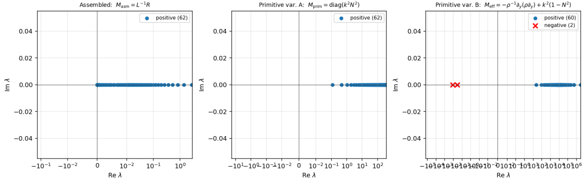
Figure 5.3. Spectra of three operators on Lane–Emden n = 3/2 . Left: the assembled operator has 62 strictly positive eigenvalues on [4 \times 10^{-8}, 2.71] , the physical g-mode spectrum. Middle: the pointwise surrogate is positive but stretches to \sim 367 — the norm gap of Proposition 1. Right: the reduced operator M_{\text{eff}} of (5.3) carries two negative eigenvalues (red crosses) in addition to a positive branch extending to 3 \times 10^6 .
