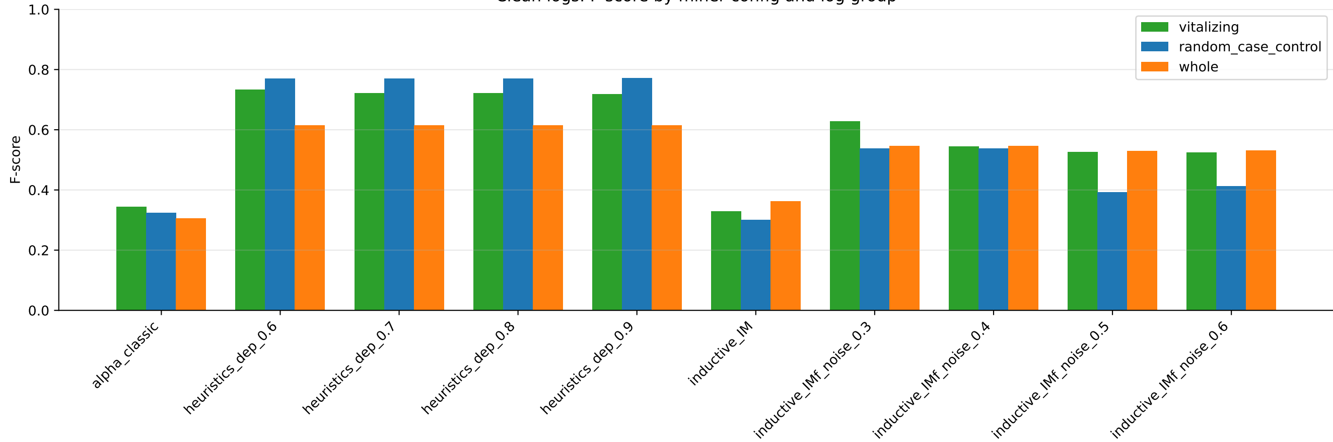
Clean logs: F-score by miner config and log group
