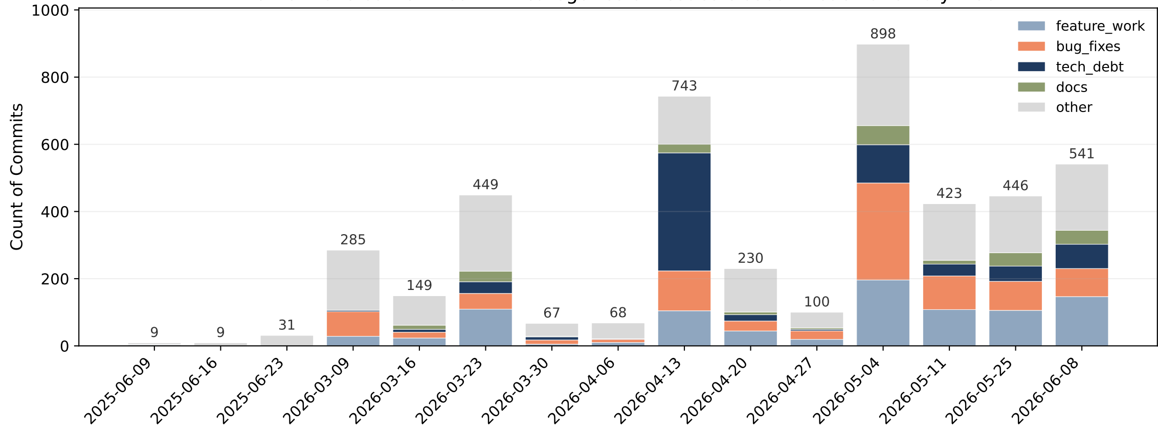
Interventions context: commit categories on issues closed in each anomaly week
