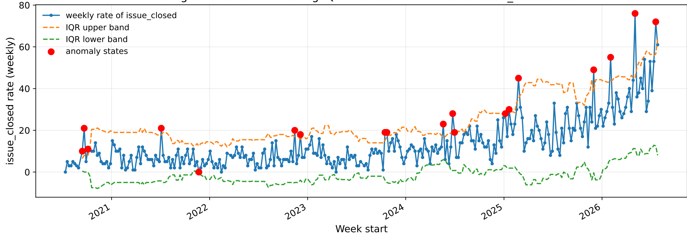
Finding anomalies with Rolling IQR method with k=1.5 for issue_closed rate
