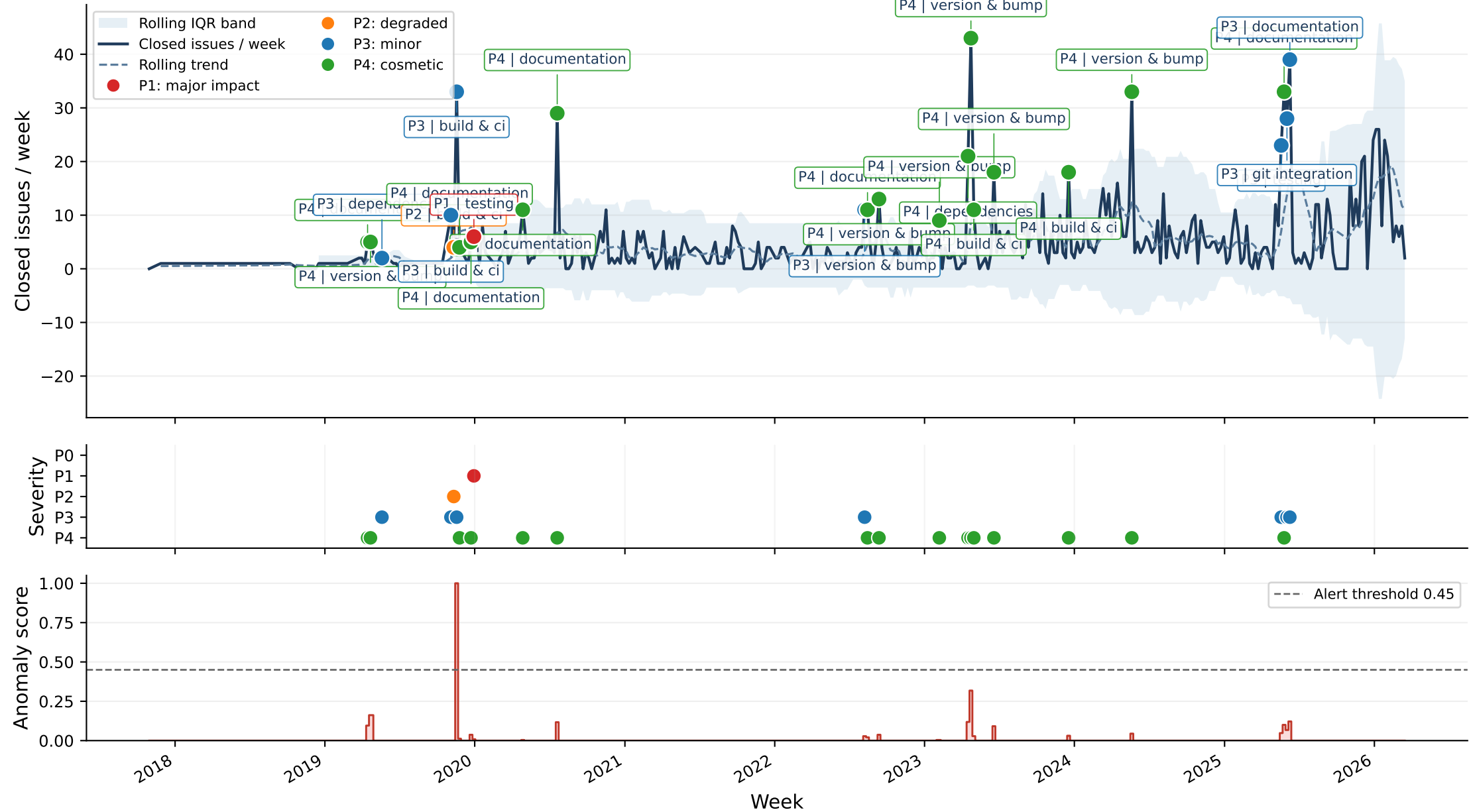
Weekly closed issues with rolling-IQR anomalies and severity context
