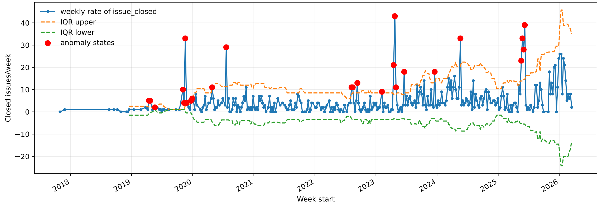
Rolling IQR anomalies with k=1.5
