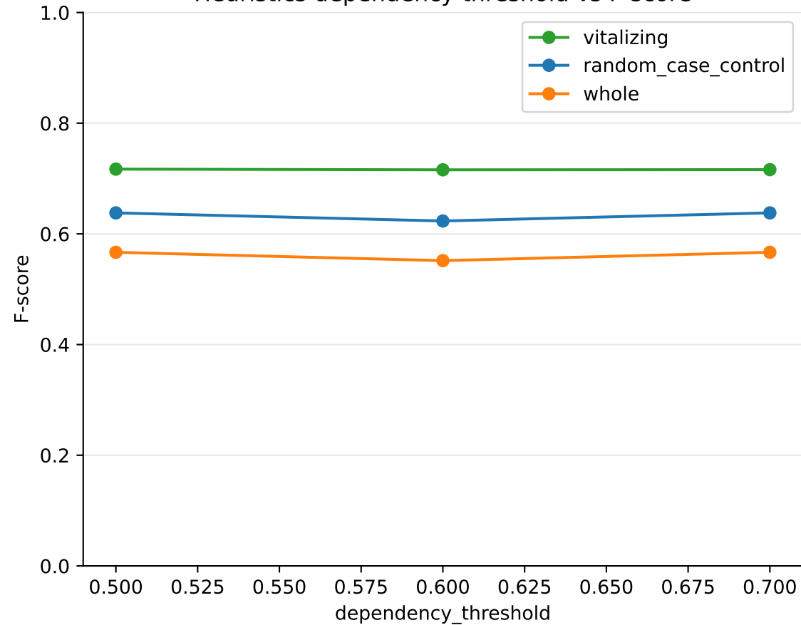
Heuristics dependency threshold vs F-score
