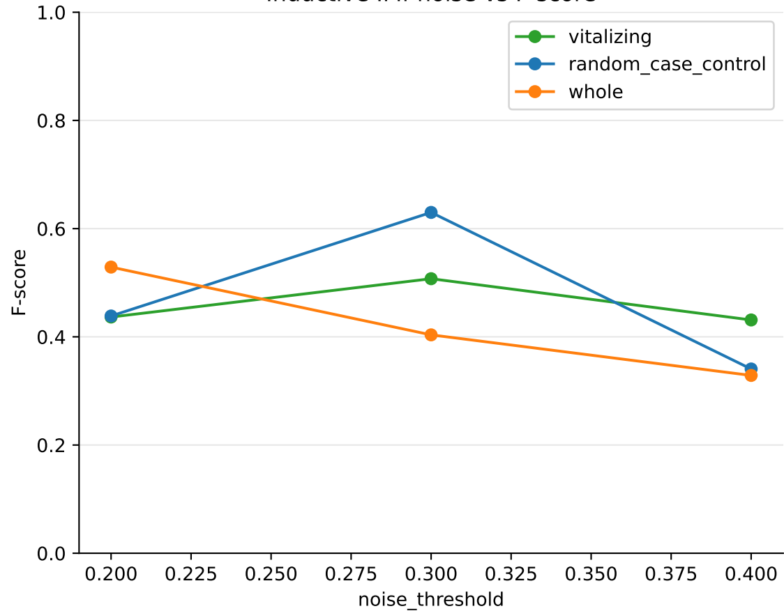
Inductive IMf noise vs F-score
