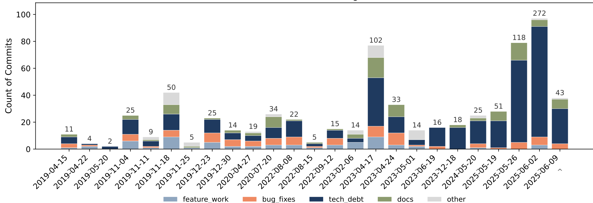
Interventions context: commit categories in each state
