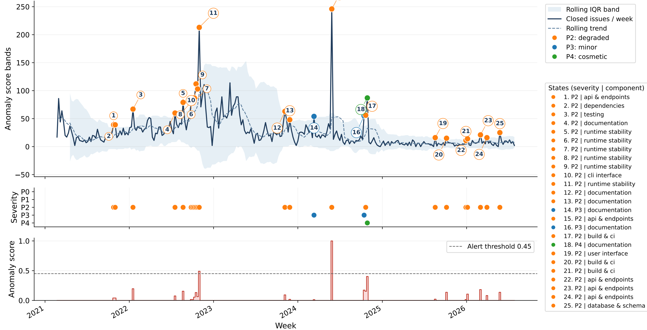
Weekly issue_closed rate with rolling-IQR anomalies and severity context
