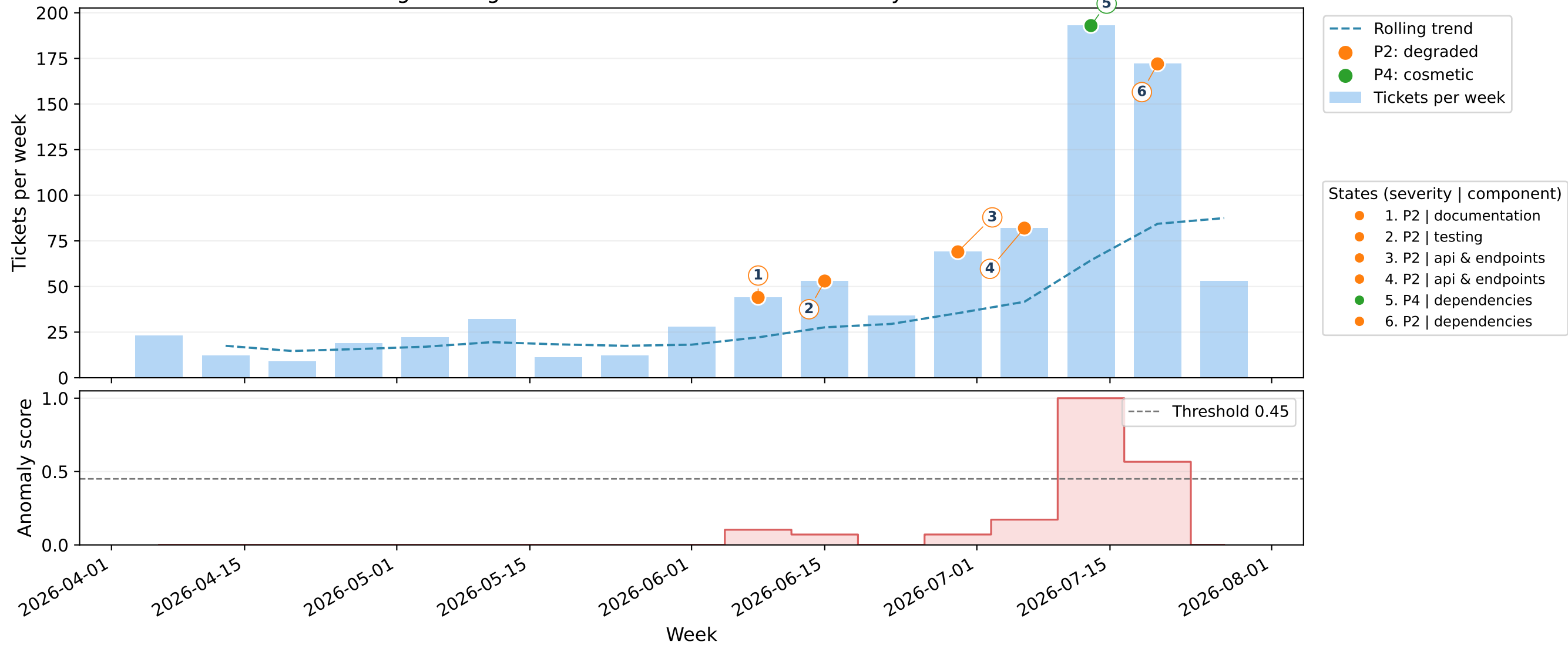
Engineering ticket volume - multimodal anomaly detection
