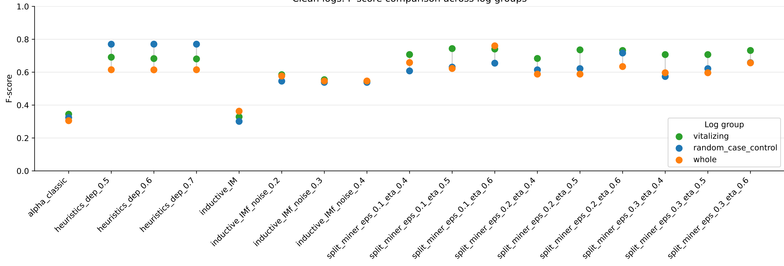
Clean logs: F-score comparison across log groups
