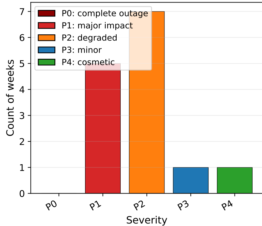
Severity distribution
