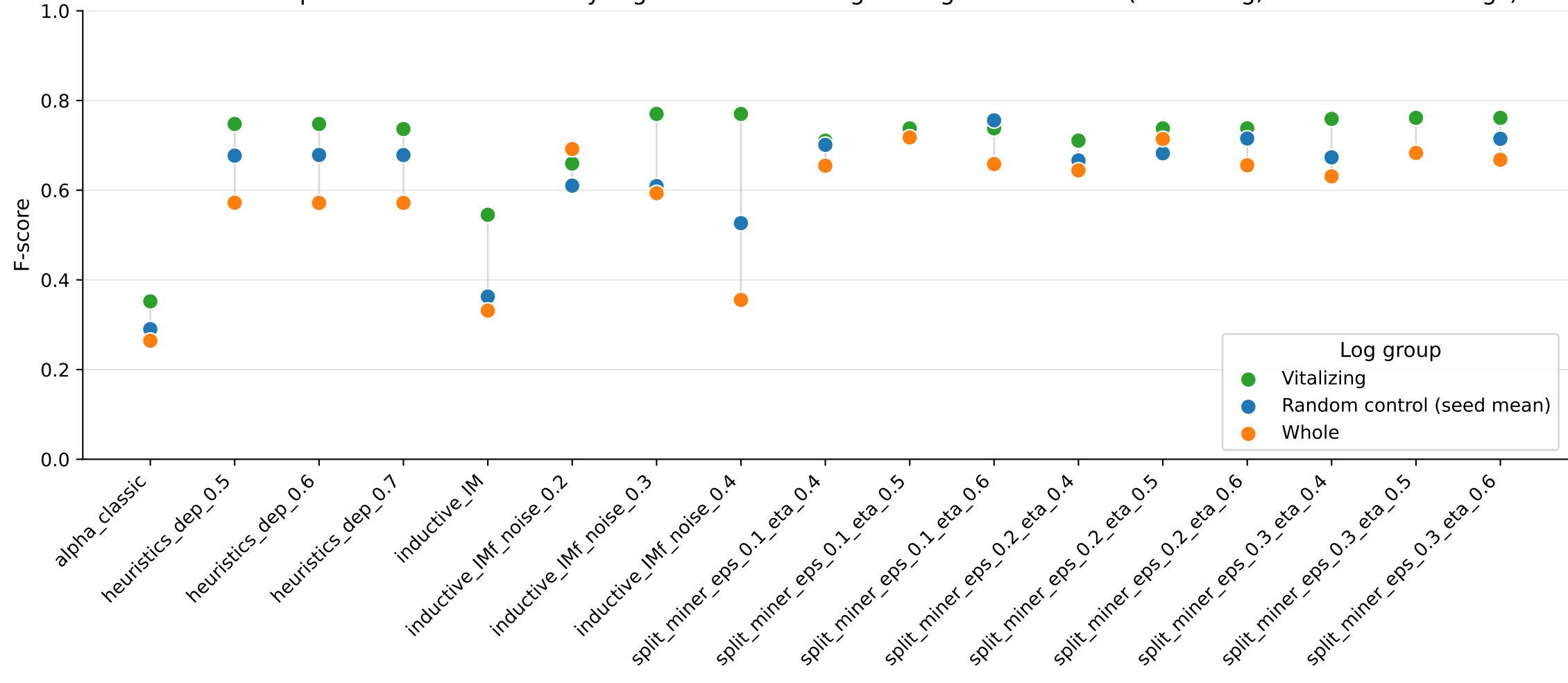
F1-Score Comparison Across Discovery Algorithms: Vitalizing Sublog vs. Baselines (Whole log; 10 Random sublogs)
