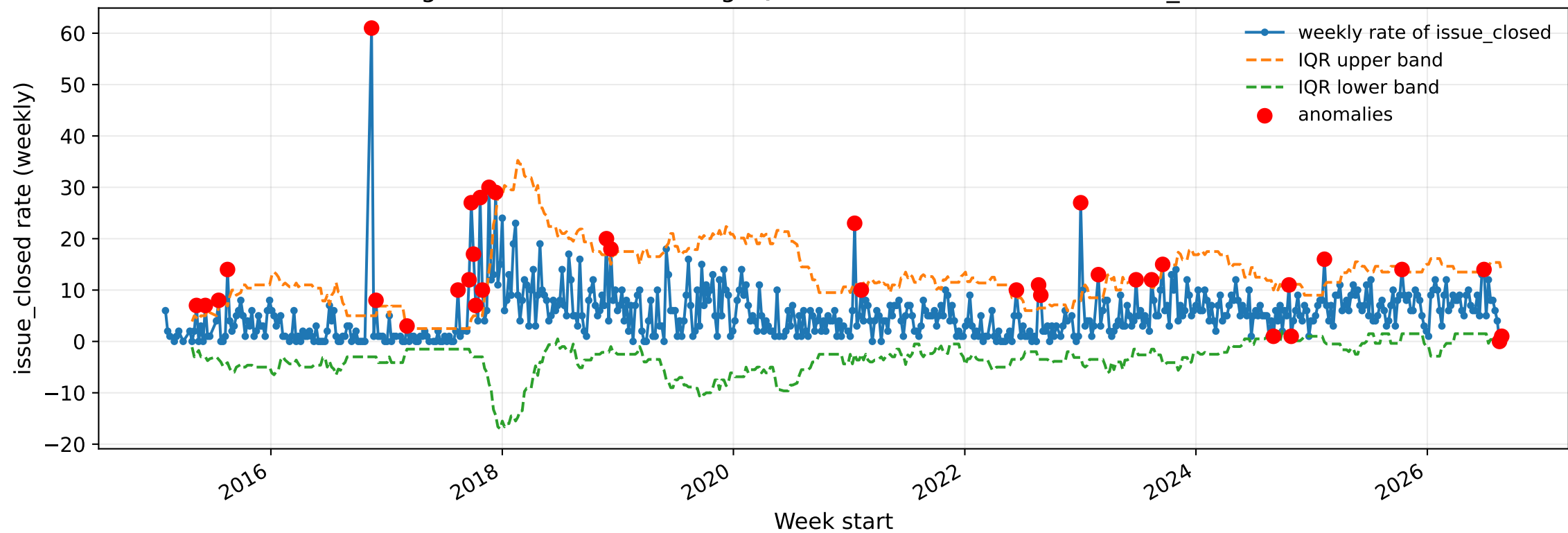
Finding anomalies with Rolling IQR method with k=1.5 for issue_closed rate
