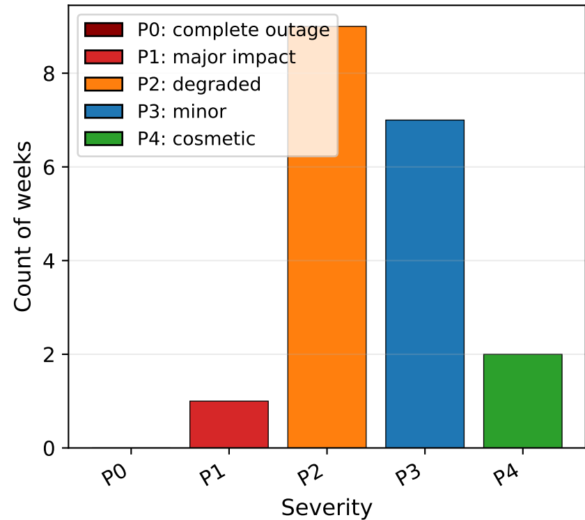
Severity distribution
