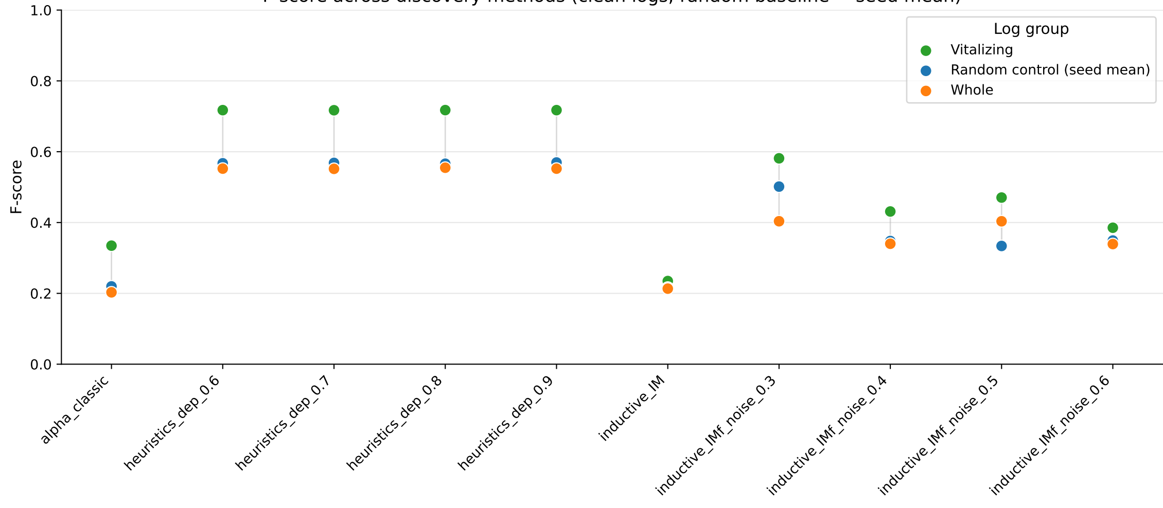
F-score across discovery methods (clean logs; random baseline = seed mean)
