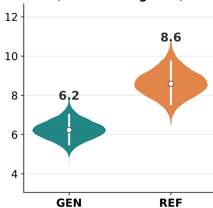
(b) Time-explicit static (SSP2-PkBudg1000)
