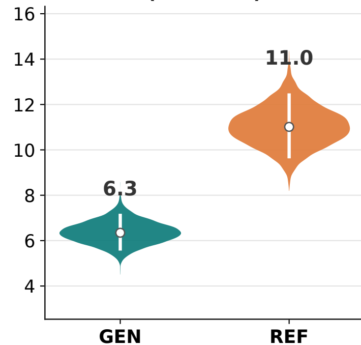
(c) Dynamic climate (IPCC AR6)
