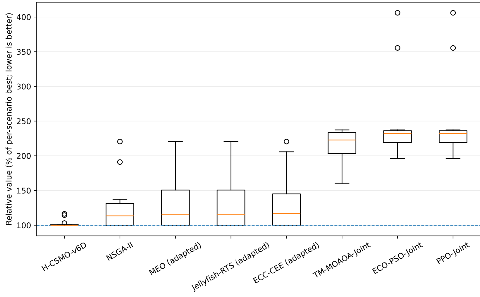
Gross carbon distribution - SLA-constrained stress
