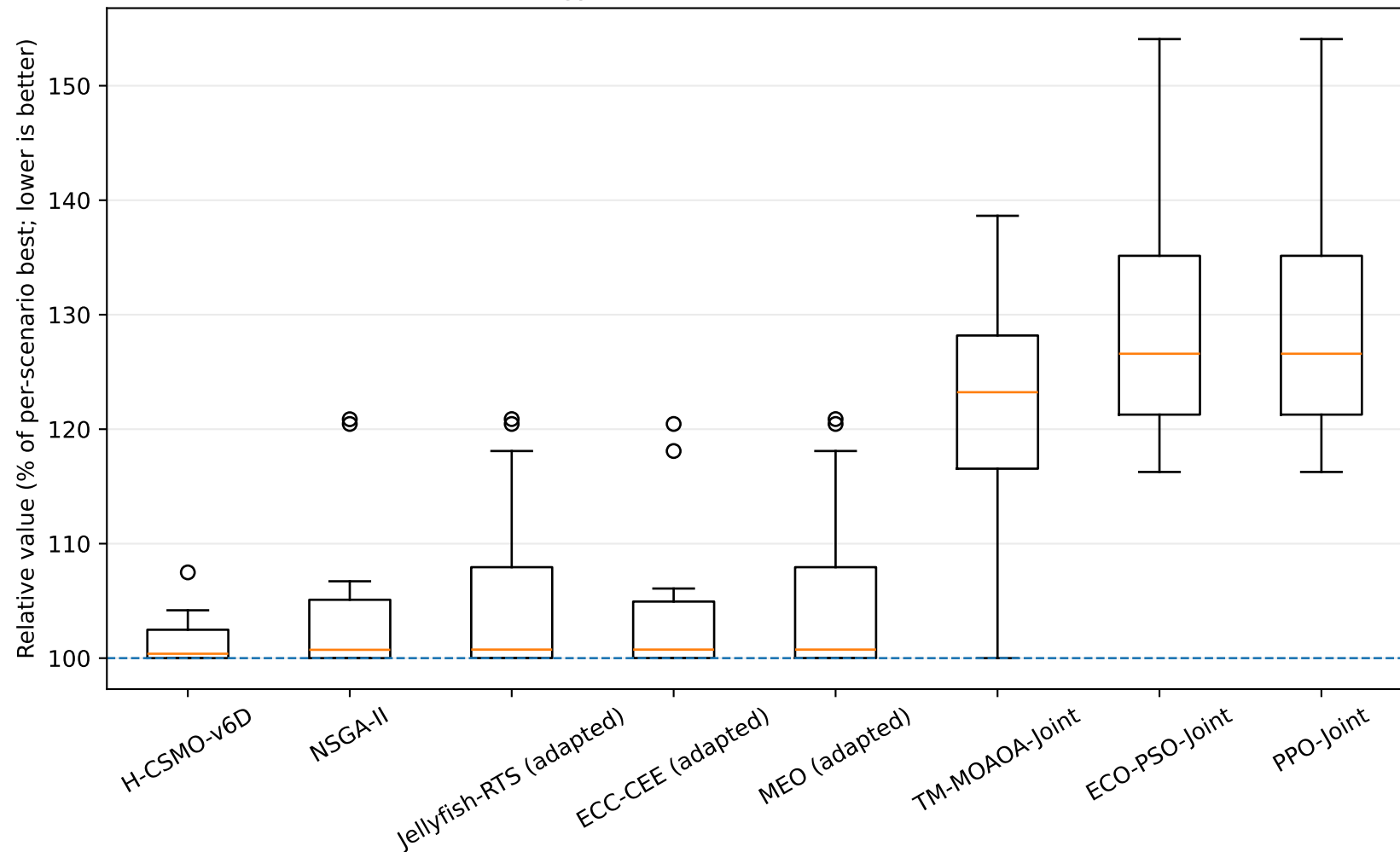
Gross energy distribution - SLA-constrained stress
