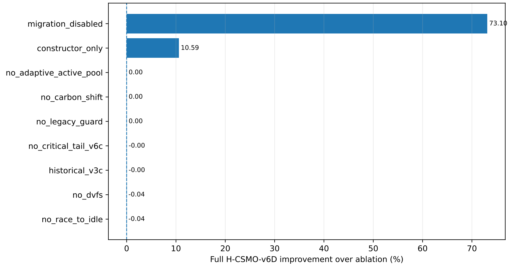
Ablation contribution - Gross carbon
