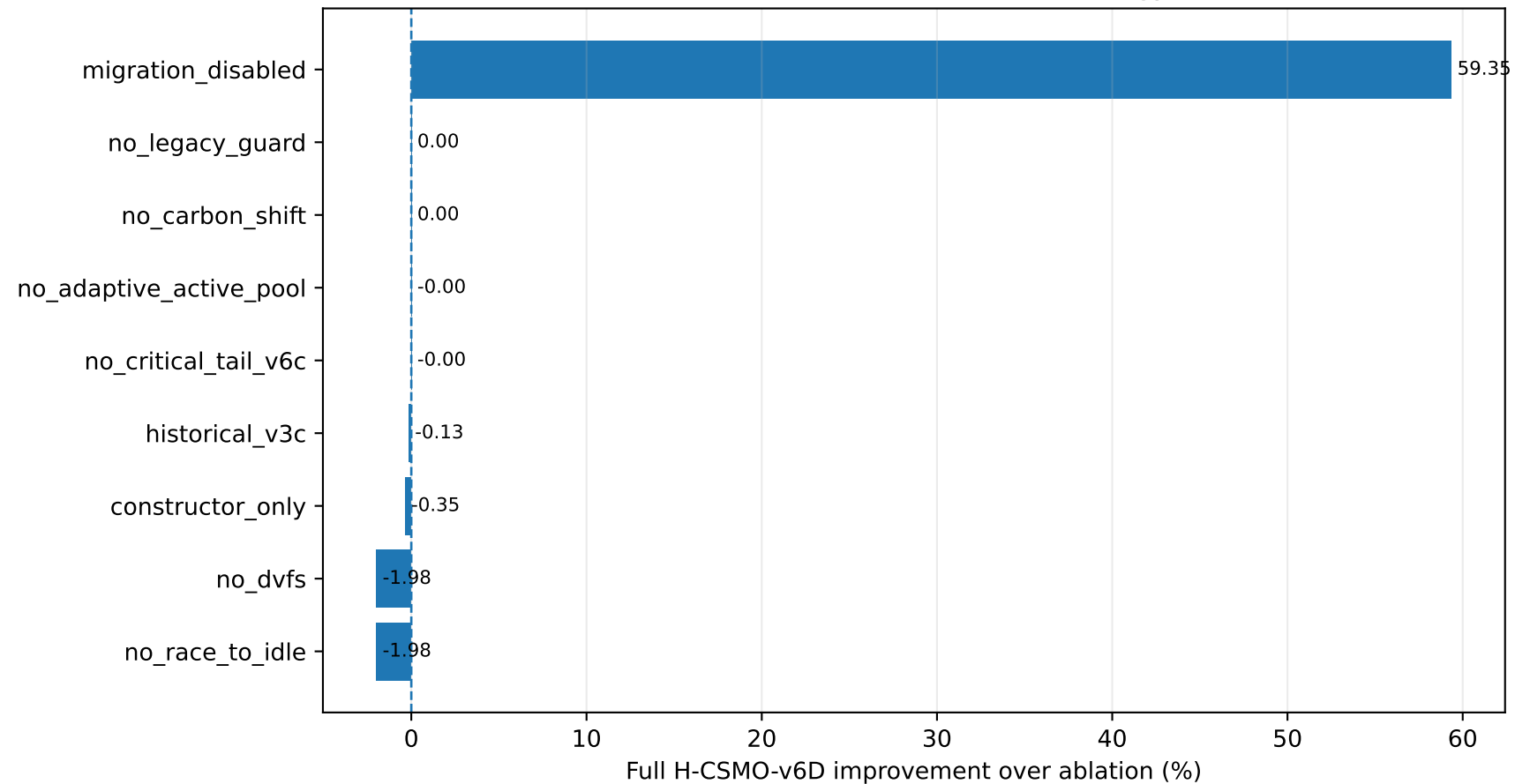
Ablation contribution - Gross energy
