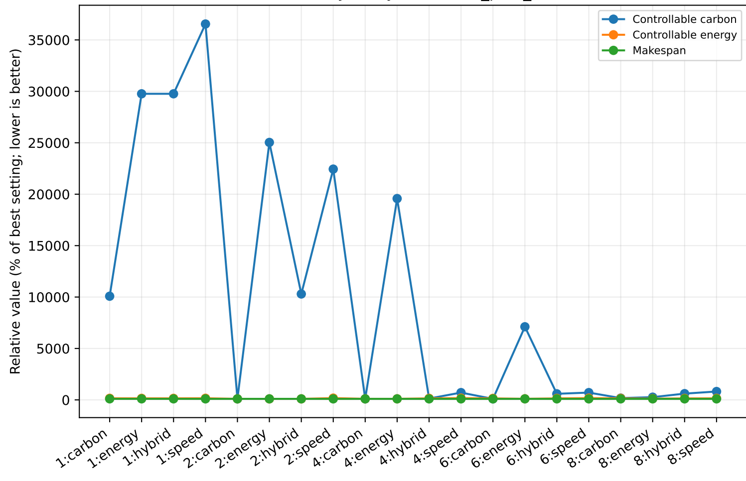
Sensitivity analysis - active_pool_size
