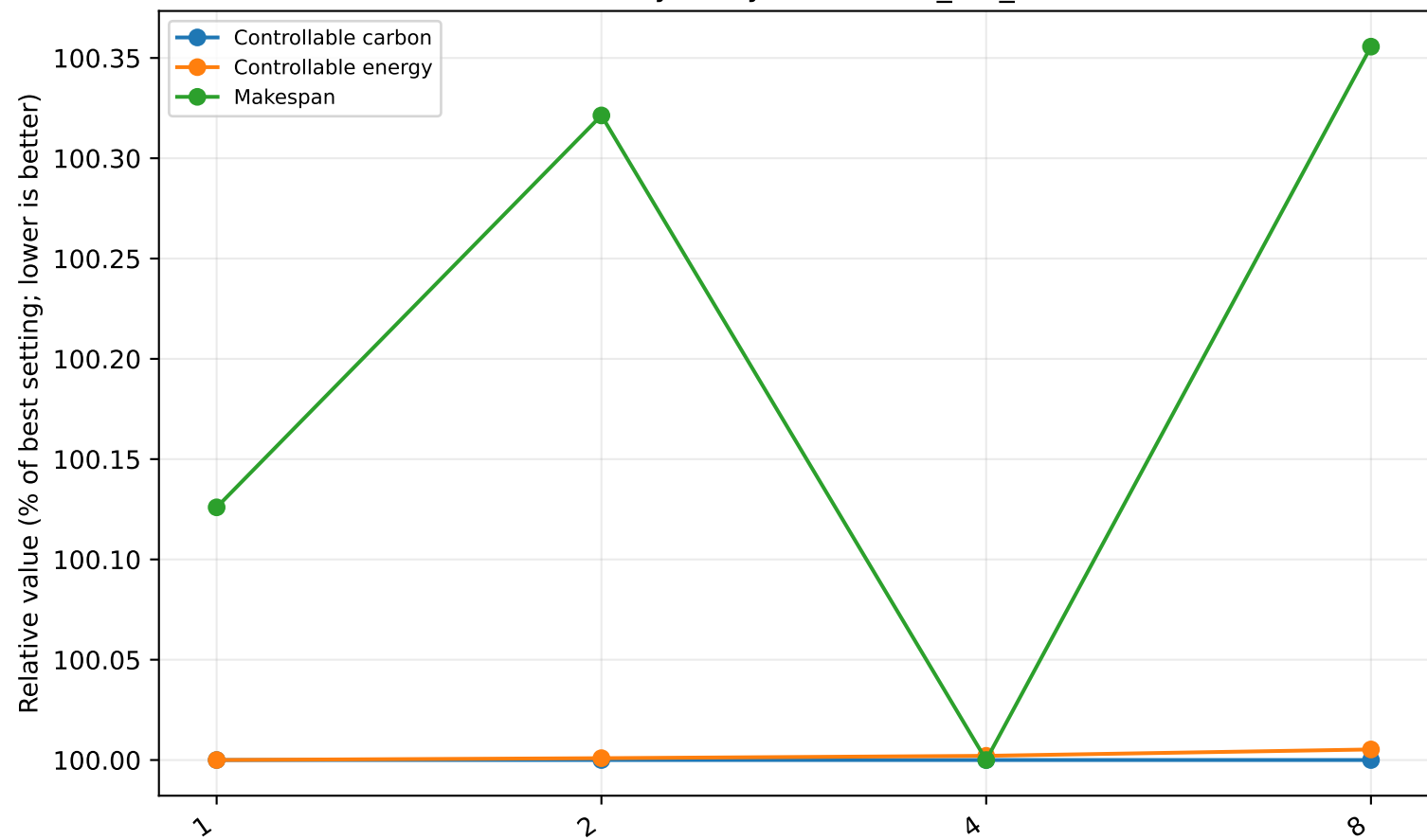
Sensitivity analysis - critical_tail_size
