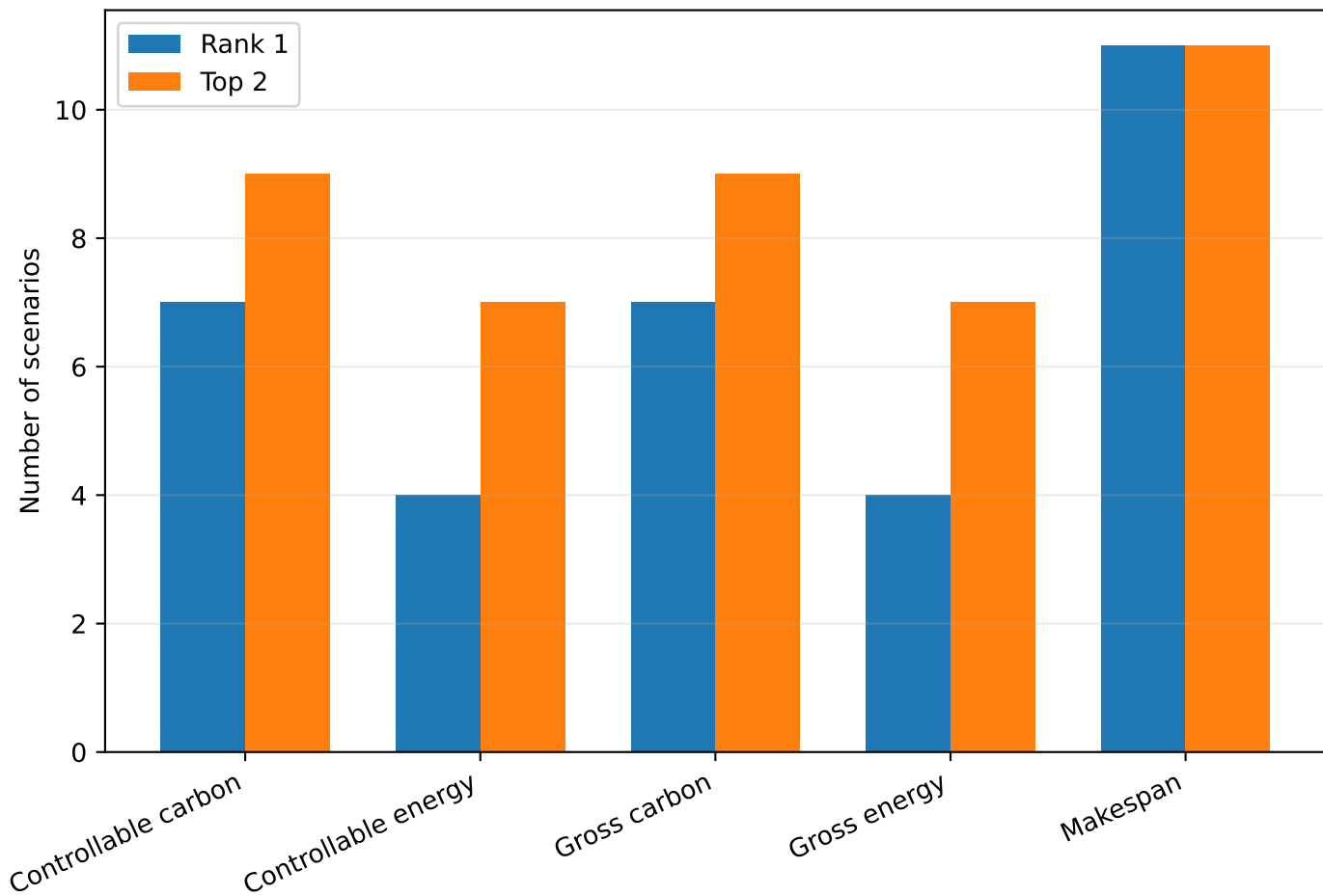
H-CSMO-v6D rank counts - SLA-constrained stress
