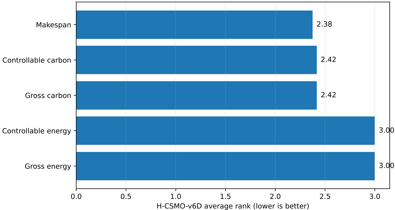
H-CSMO-v6D rank by metric - SLA-constrained stress
