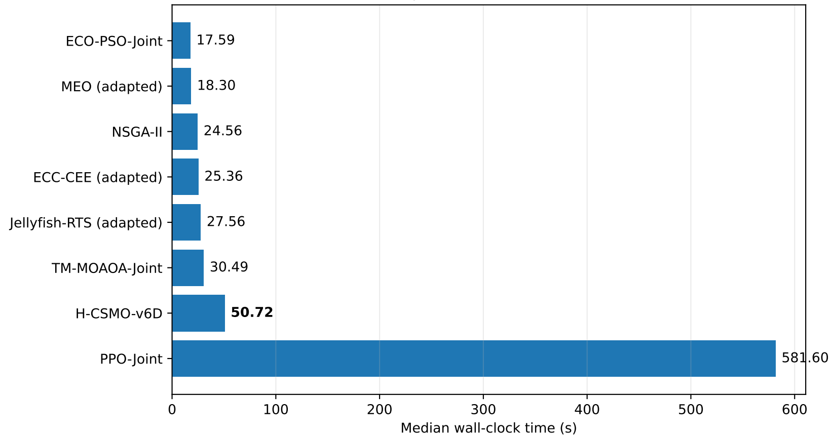
Runtime comparison - SLA-constrained stress
