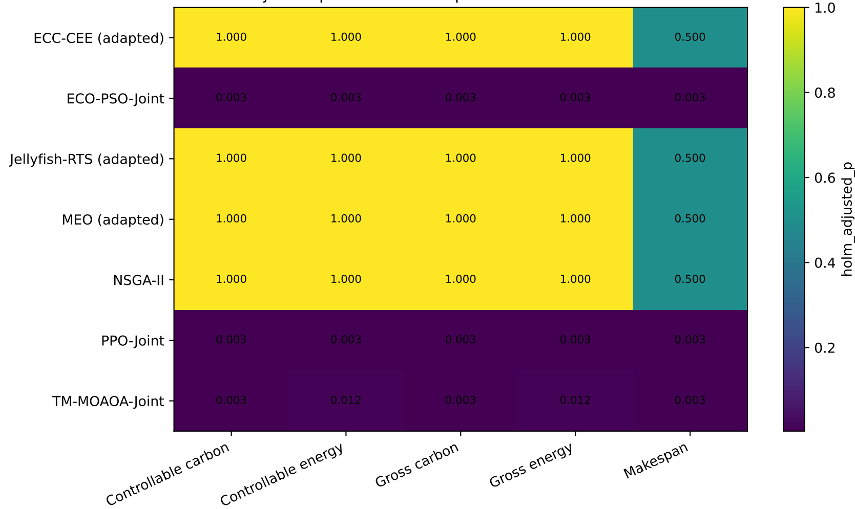
Holm-adjusted paired Wilcoxon p-values - SLA-constrained stress
