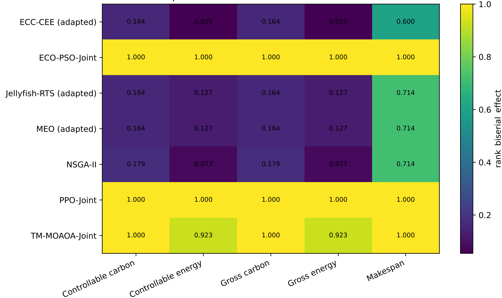
Matched-pairs rank-biserial effects - SLA-constrained stress
