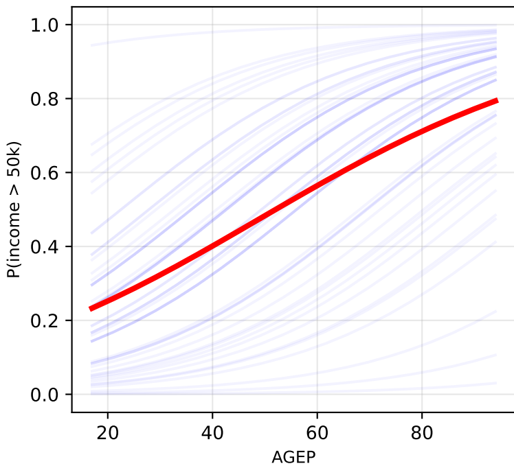
AGEP
