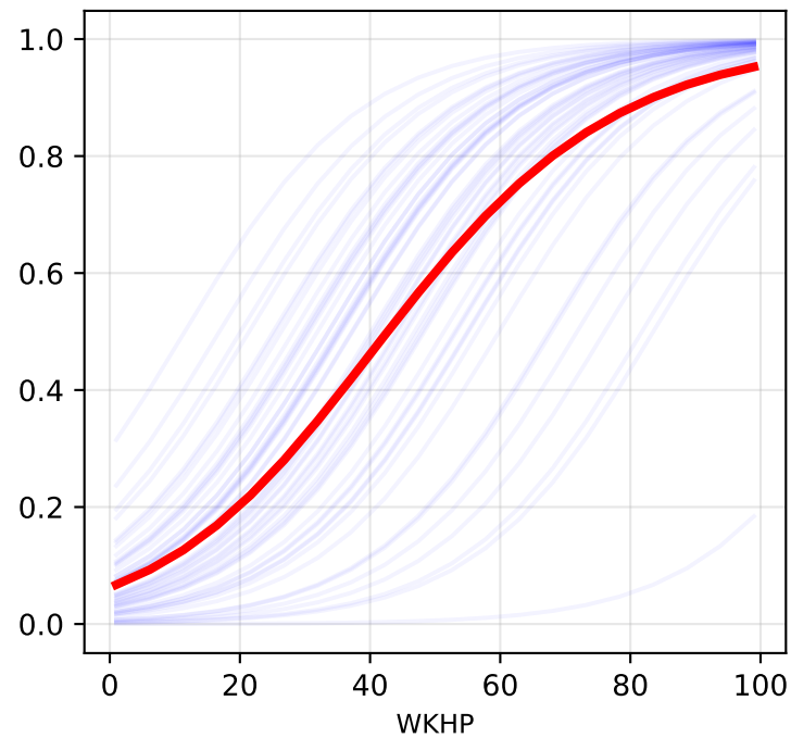
WKHP
