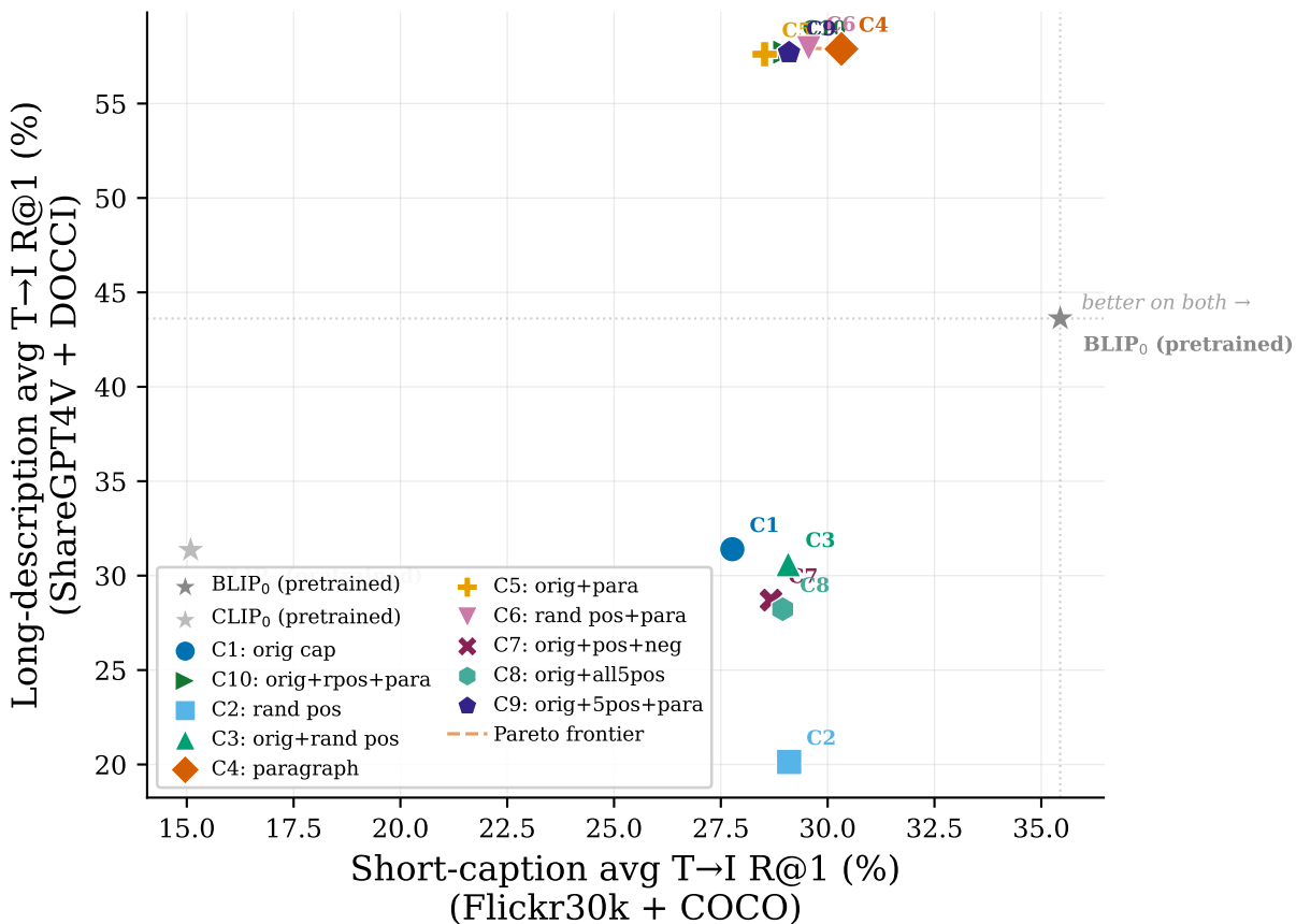
Trade-off: short-caption vs. long-description retrieval (T→I)
