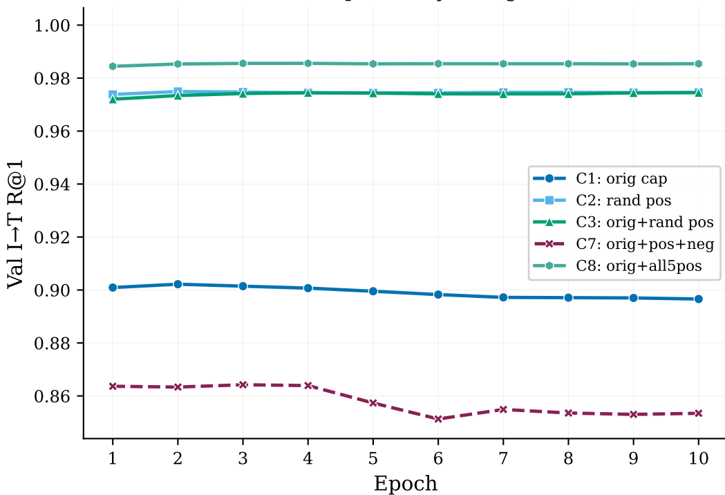
(a) Caption-only configs
